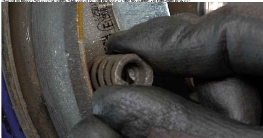
39 Monteer de borgveer.
